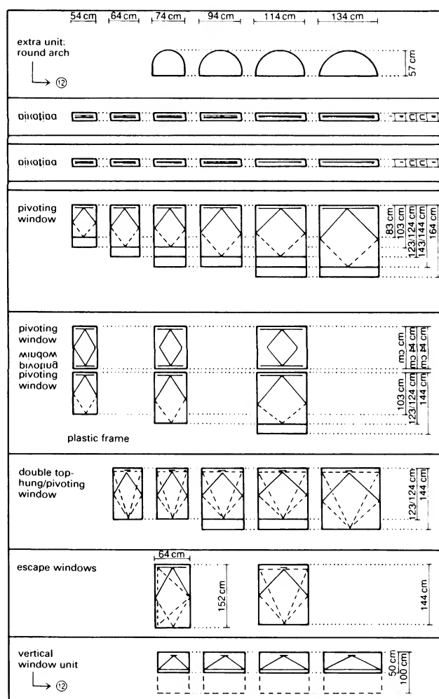
⑩ Window sizes
